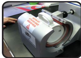
Step 3 Using mug press apply required time (140 secs) heat (190°C/370°F) and normal pressure.
